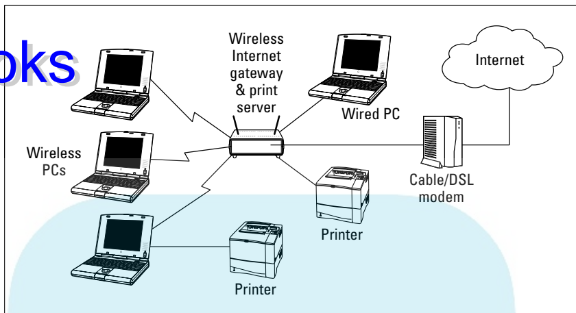
Figure 4-4: Look for a wireless gateway that combines AP, DHCP, NAT, print server, and switched hub functions in one unit.
